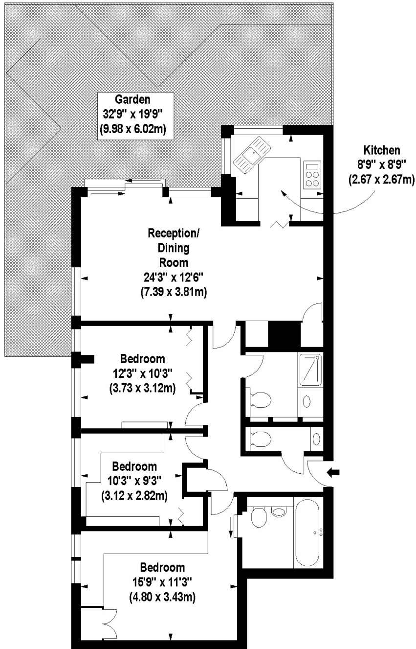
First Floor
